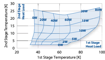
RDE-418D4 Cold Head Capacity Map (60 Hz)
