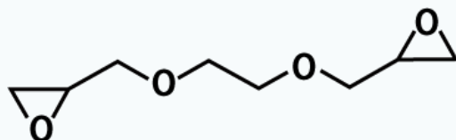
Ethylene Glycol Diglycidyl Ether
