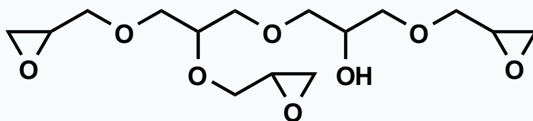
Diglycerol Polyglycidyl Ether
