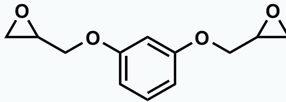
Resorcinol Diglycidyl Ether
