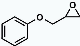
Phenyl Glycidyl Ether
