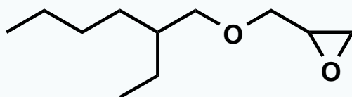
2-Ethylhexyl Glycidyl Ether
